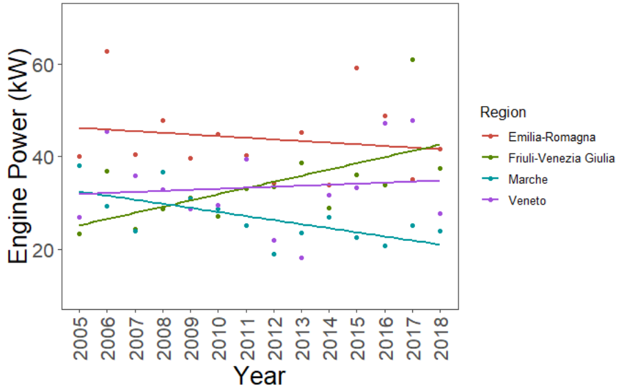
Figure 10. Trends in the mean engine power of SSF vessels in the four Italian regions involved in the project for the period 2005-2018.
