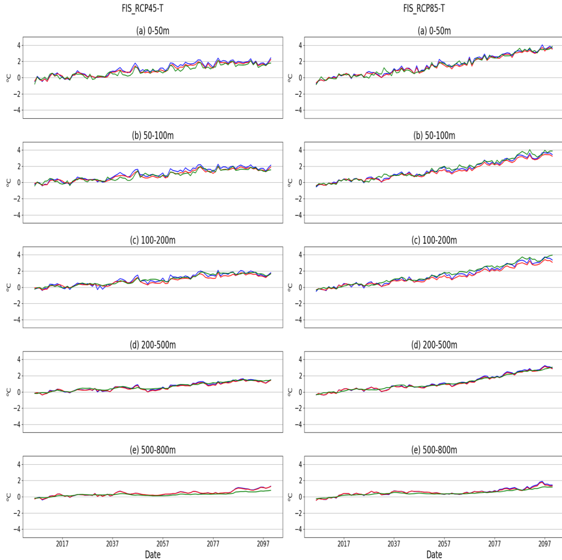
Figure 8 - Annual time series of temperature anomaly (°C) in the three offshore (deeper than 200 m) areas of the Adriatic-Ionian Sea: GSA17 - northern Adriatic (blue), GSA18 - southern Adriatic (red) and GSA19 - Ionian (green). Time series cover the 2005-2099 period for the two emission RCP4.5 (left) and RCP8.5 (right) scenarios.
