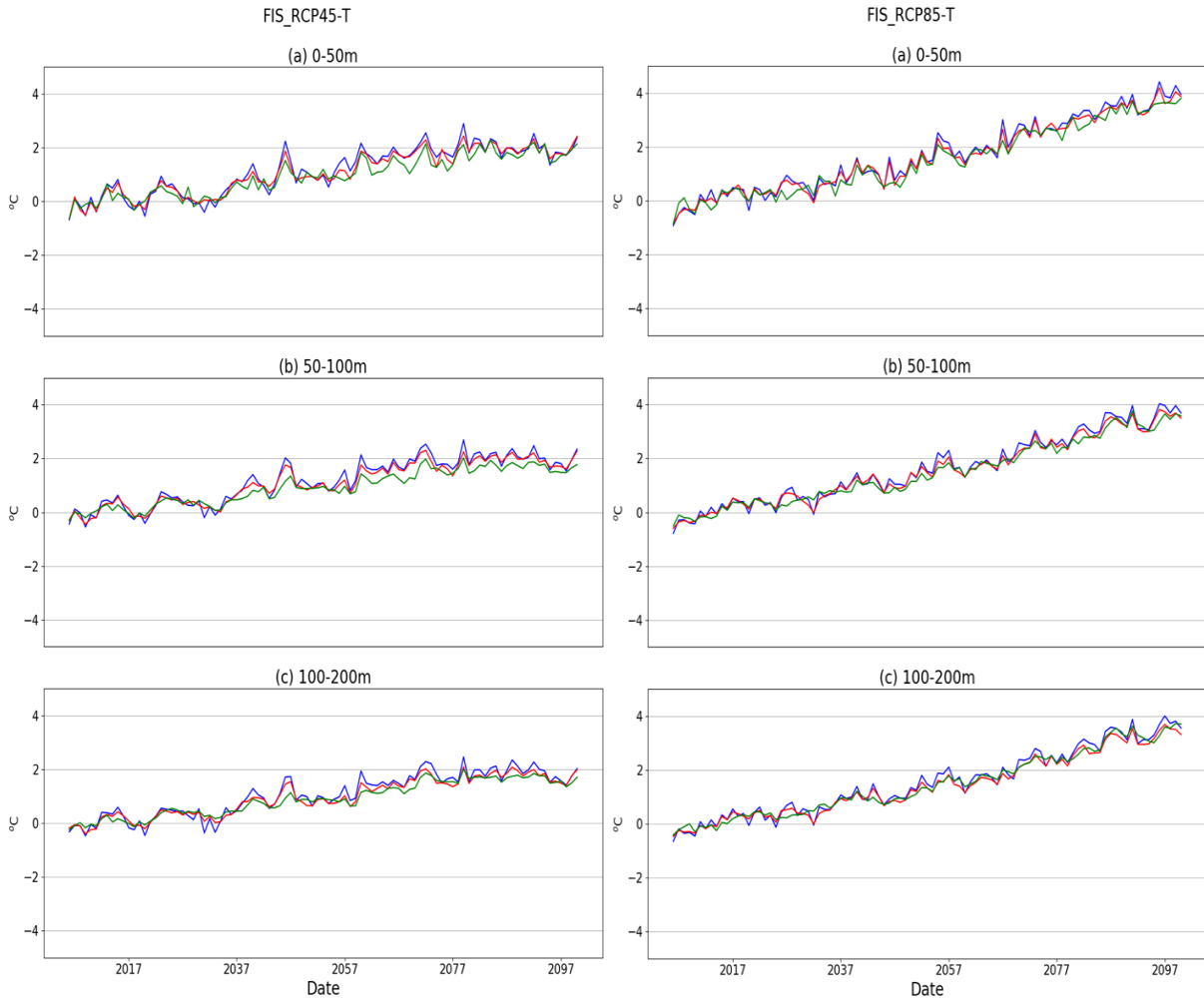
Figure 7 - Annual time series of temperature anomaly (°C) in the three inshore (depth less than 200 m) areas of the Adriatic-Ionian Sea: GSA17 - northern Adriatic (blue), GSA18 - southern Adriatic (red) and GSA19 - Ionian (green). Time series cover the 2005-2099 period for the two emission RCP4.5 (left) and RCP8.5 (right) scenarios.
