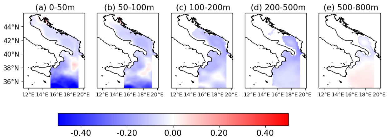
Figure 13 - Mean salinity anomaly in the MID-FUTURE of the RCP4.5 scenario in the five layers: 0-50 m, 50-100 m, 100-200 m, 200-500 m and 500-800 m.
