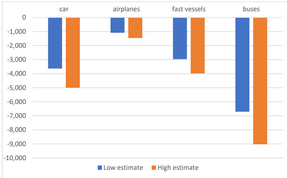
Fig. 17: Yearly variation of CO2 (in tons.) expected for 1% Italy-Croatia travellers shifting from liners to other means of transport at 2030 travellers flows (e.g. 1% travellers use cars/airplanes/buses instead of liners)
