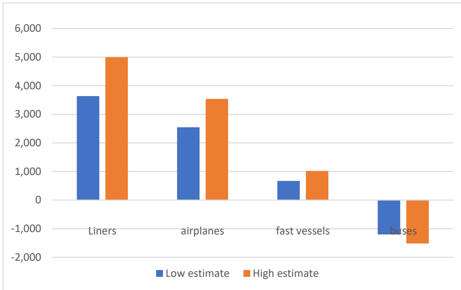
Fig. 16: Yearly variation of CO2 (in tons.) expected for 1% Italy-Croatia travellers shifting from cars to other means of transport at 2030 travellers flows (e.g. 1% travellers use ships/airplanes/buses instead of cars)
