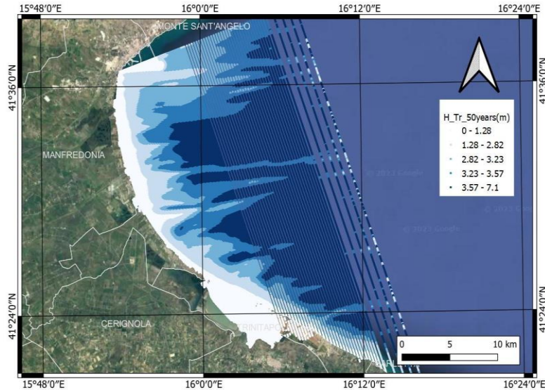
Fig. 16. Flooding scenario for 50y return period
