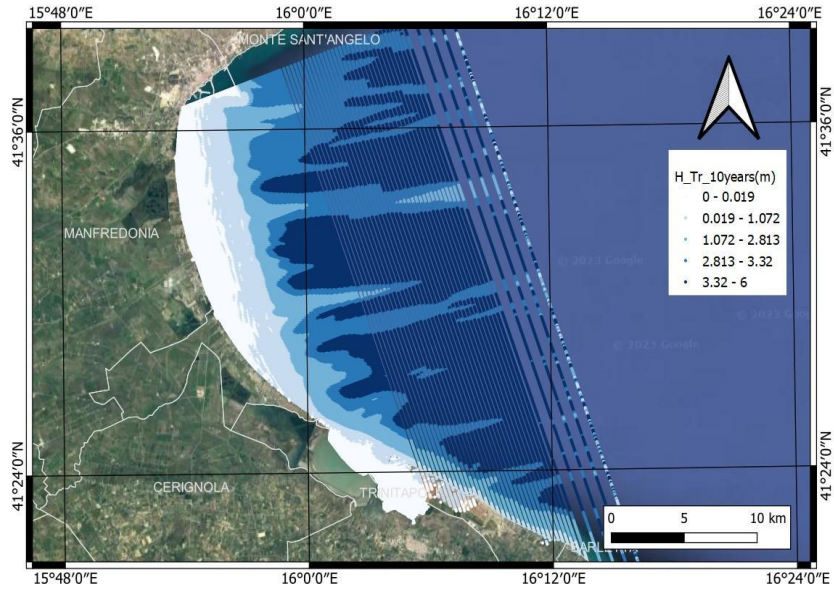
Fig. 14. Flooding scenario for 10y return period
