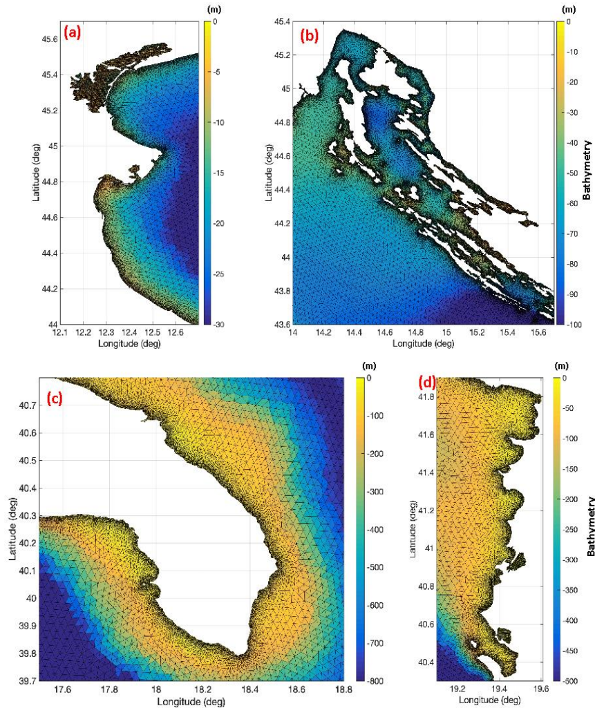
Fig. 8: Enlarged views (bathymetry and grid) in coastal zones of high resolution coastal modelling for Adriatic Sea
