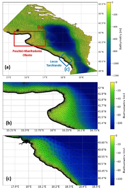
Fig. 9: Geographical domain, bathymetry and grid of very high-resolution coastal model SOAP for Apulia Pilots
