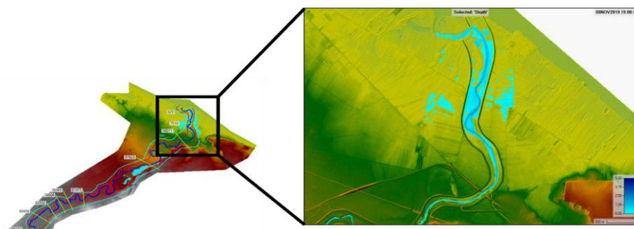
Fig. 17. Ofanto river inland inundation in HEC RAS
