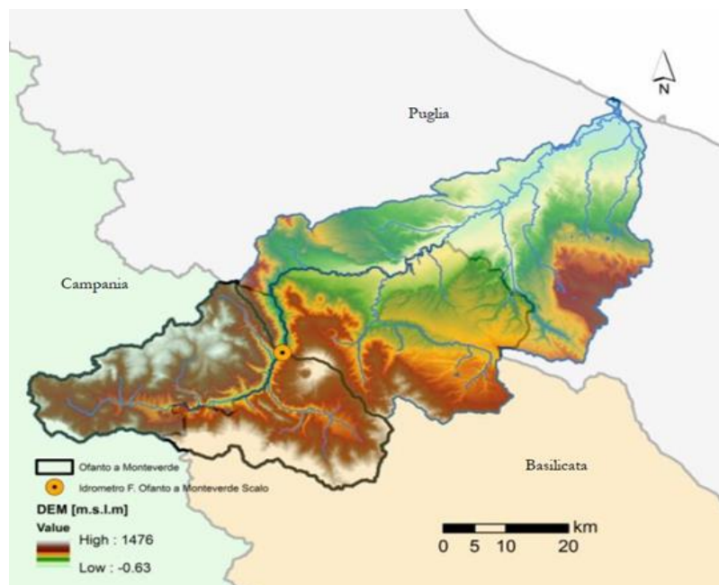
Fig. 3: Ofanto Pilot: hydrographic basin and Digital Terrain Model (DTM)
