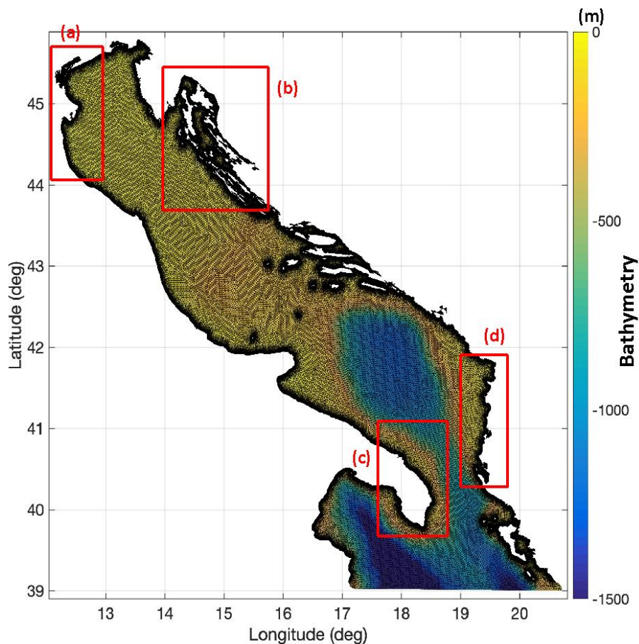
Fig. 7: Geographical domain, bathymetry and grid of high-resolution coastal model AdriFs for Adriatic Sea
