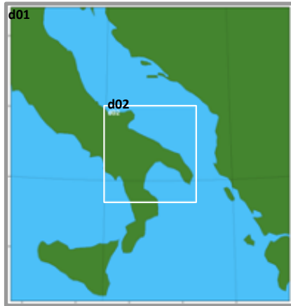
Fig. 10. The two nested WRF domains d01 and d02
