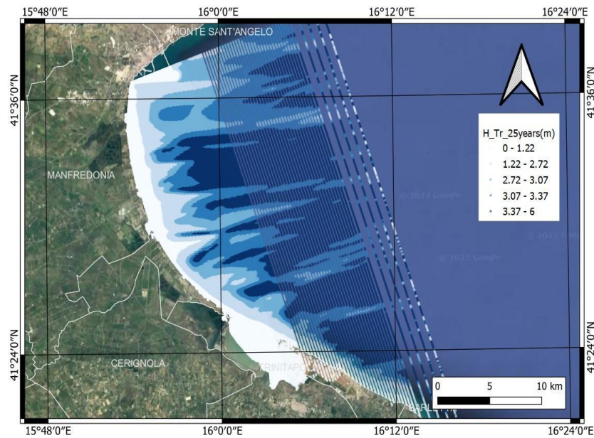
Fig. 15. Flooding scenario for 25y return period
