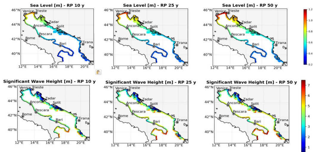
Fig. 6: Maps of sea level and significant wave height of The Adriatic Sea for the return period of 10, 25 and 50 years at the model nodes closest to the coastline
