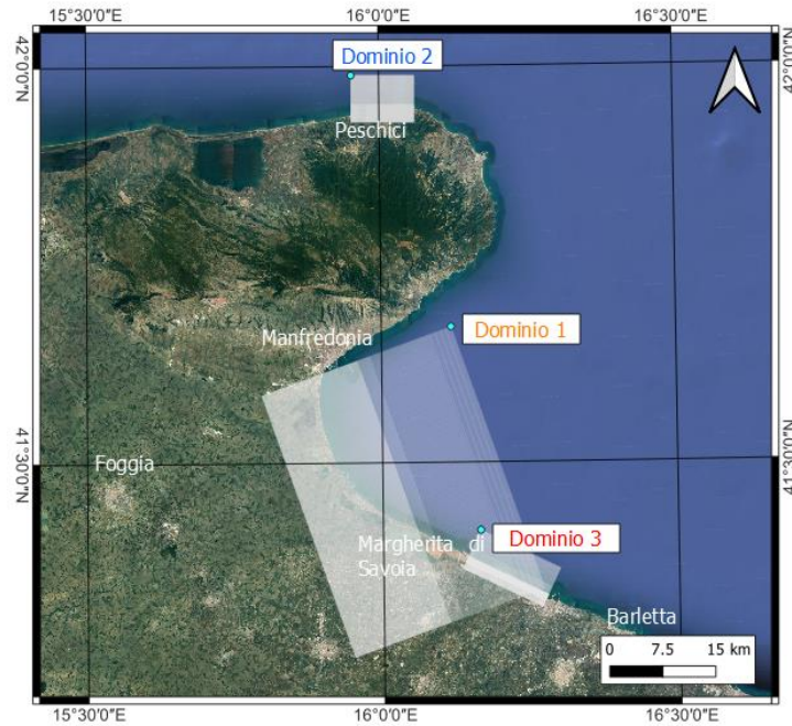
Fig. 11. Considered domains for XBeach analyses
