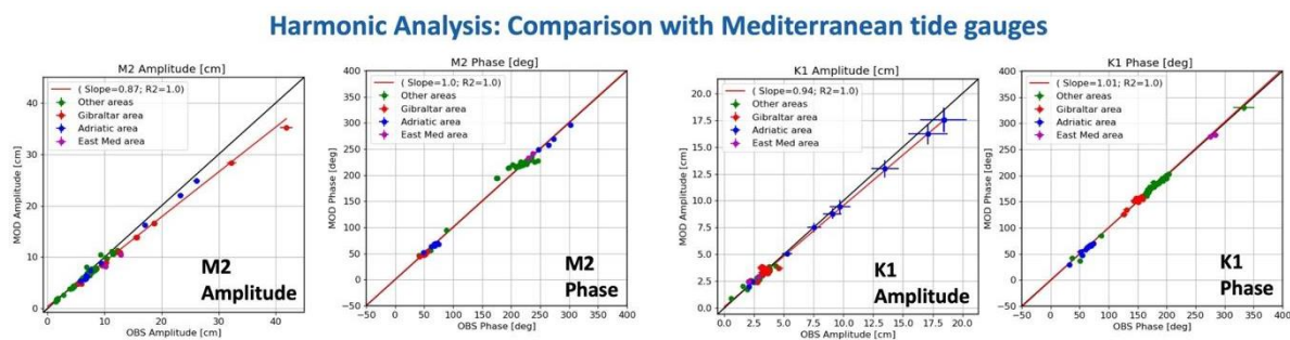
Fig. 5. Scatter plots: Model M2 and K1 tidal amplitude and phase with respect to tide gauges measurements
