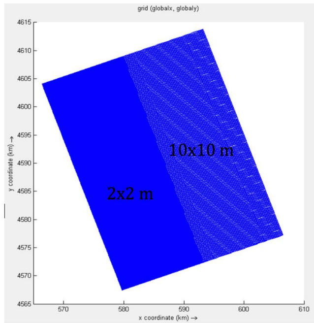
Fig. 12. Bathymetry grid domain constructed for XBeach
